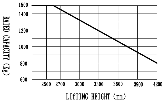
ES15-15ES RATED CAPACITIES GRAPH
